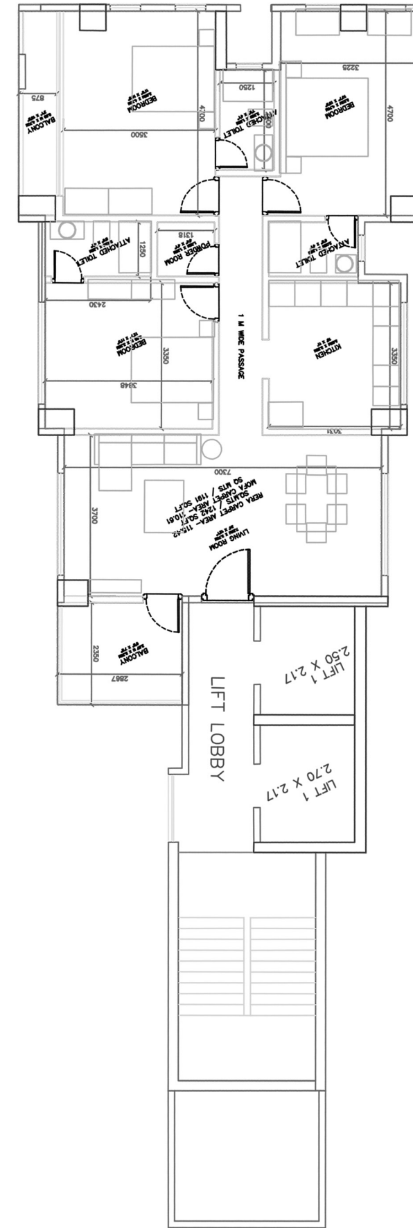
5 TH TO 13 TH FLOOR PLAN
